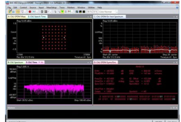
Using data acquired from S-Series, VSA shows an EVM for IEEE 802.11 QAM 64 of 0.47%.
